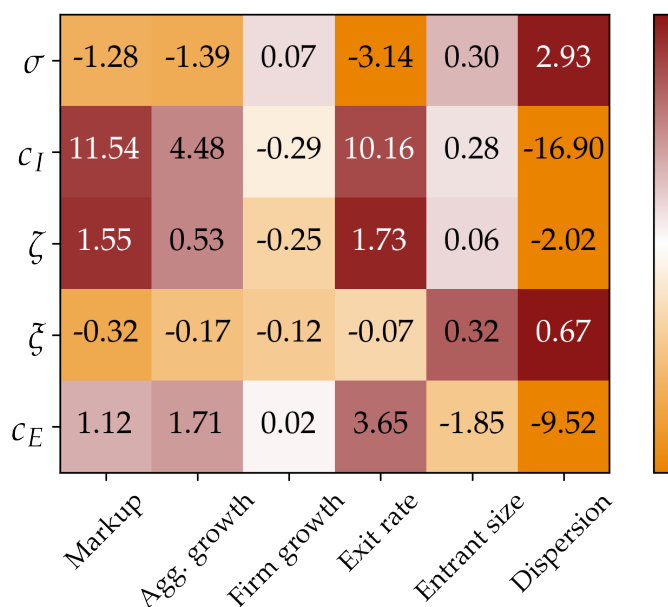
Figure B.8: Sensitivity Matrix
